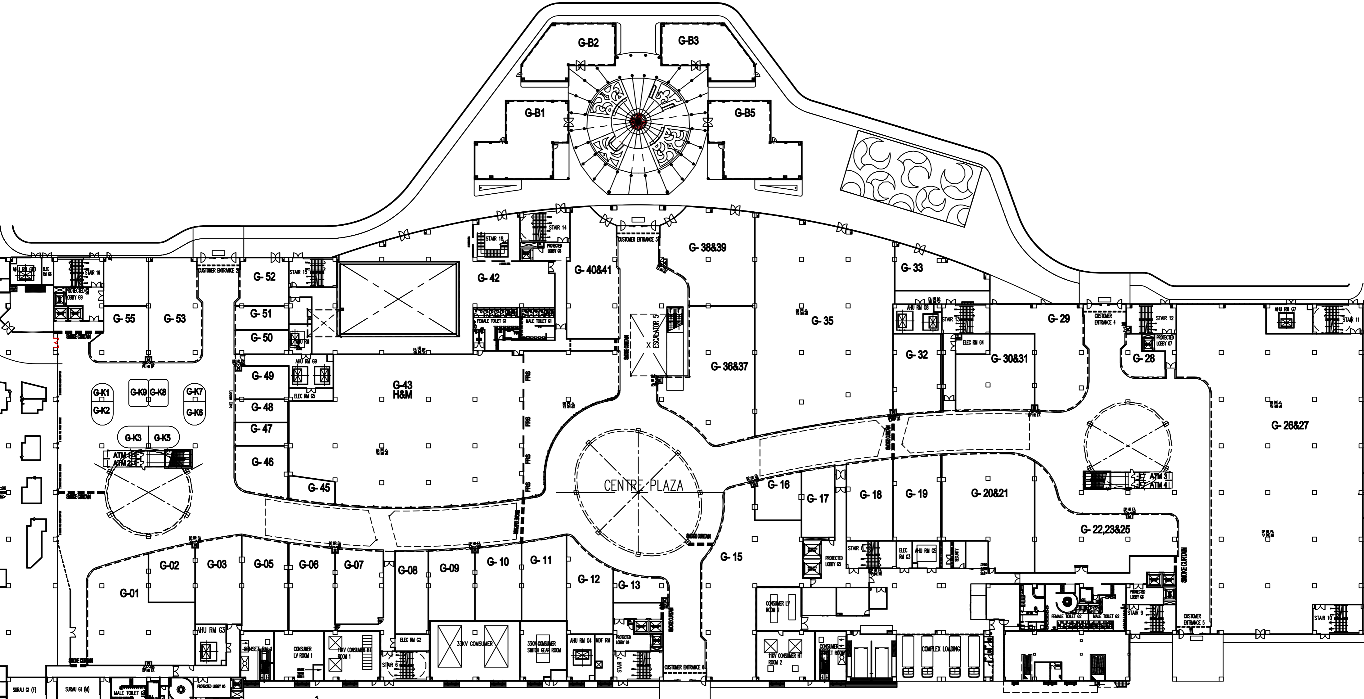
GROUND FLOOR PLAN SCALE 1:600
